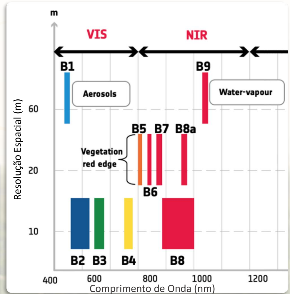
Bandas Multiespectrais Copérnico Sentinel-2
